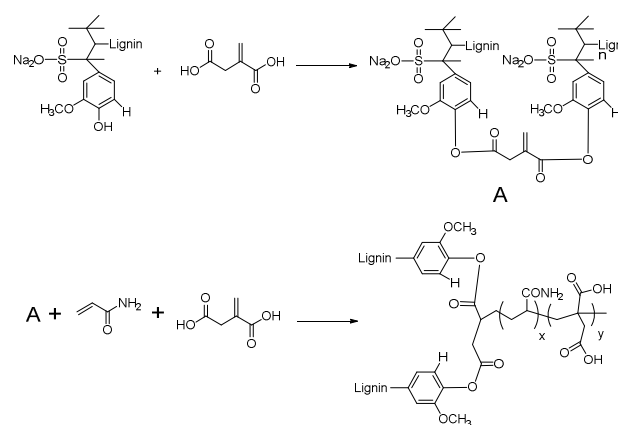
Scheme 1: Reaction route for the synthesis of lignin terpolymer (LAI).
