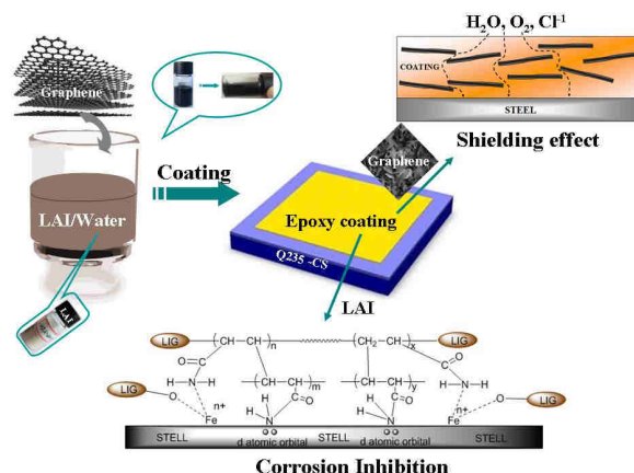
Fig.10: Schematic diagram of the anticorrosion mechanism of graphene and LAI ploymer.
